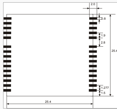
Figure 16: Recommendations for layout (JP13-LP with edge contacts).
