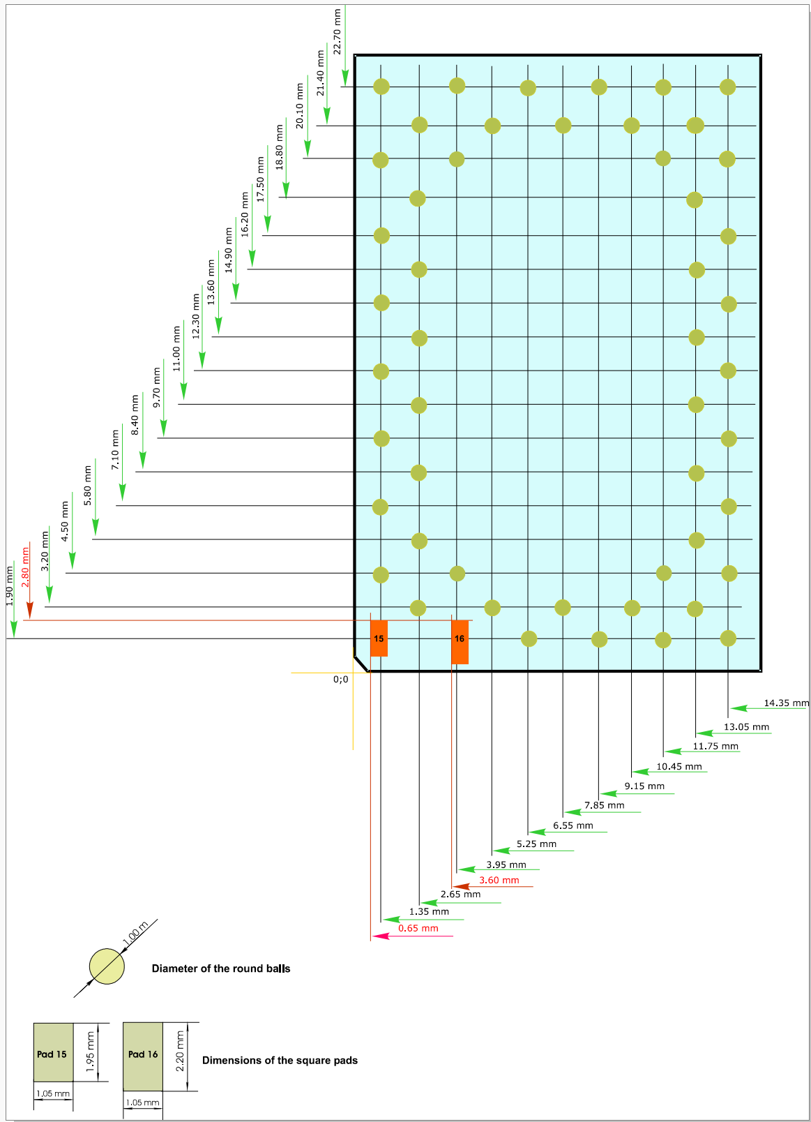
Figure 14: The mechanical draw of the JP13-S-LP receiver
