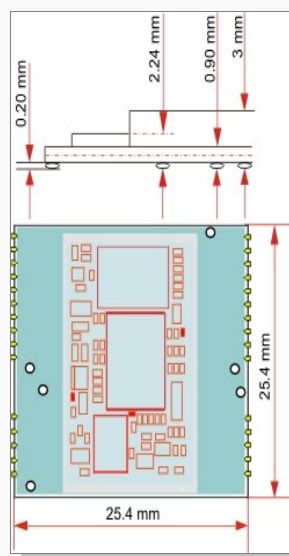
Figure 10: The mechanical draw of the JP13-LP with edge contacts
