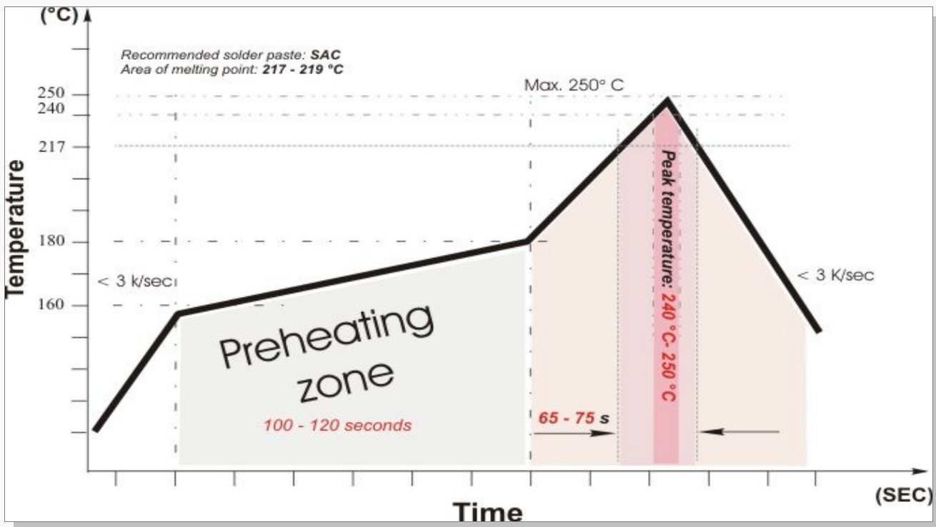
Figure 17: Typical solder conditions (temperature profile, reflow conditions).
