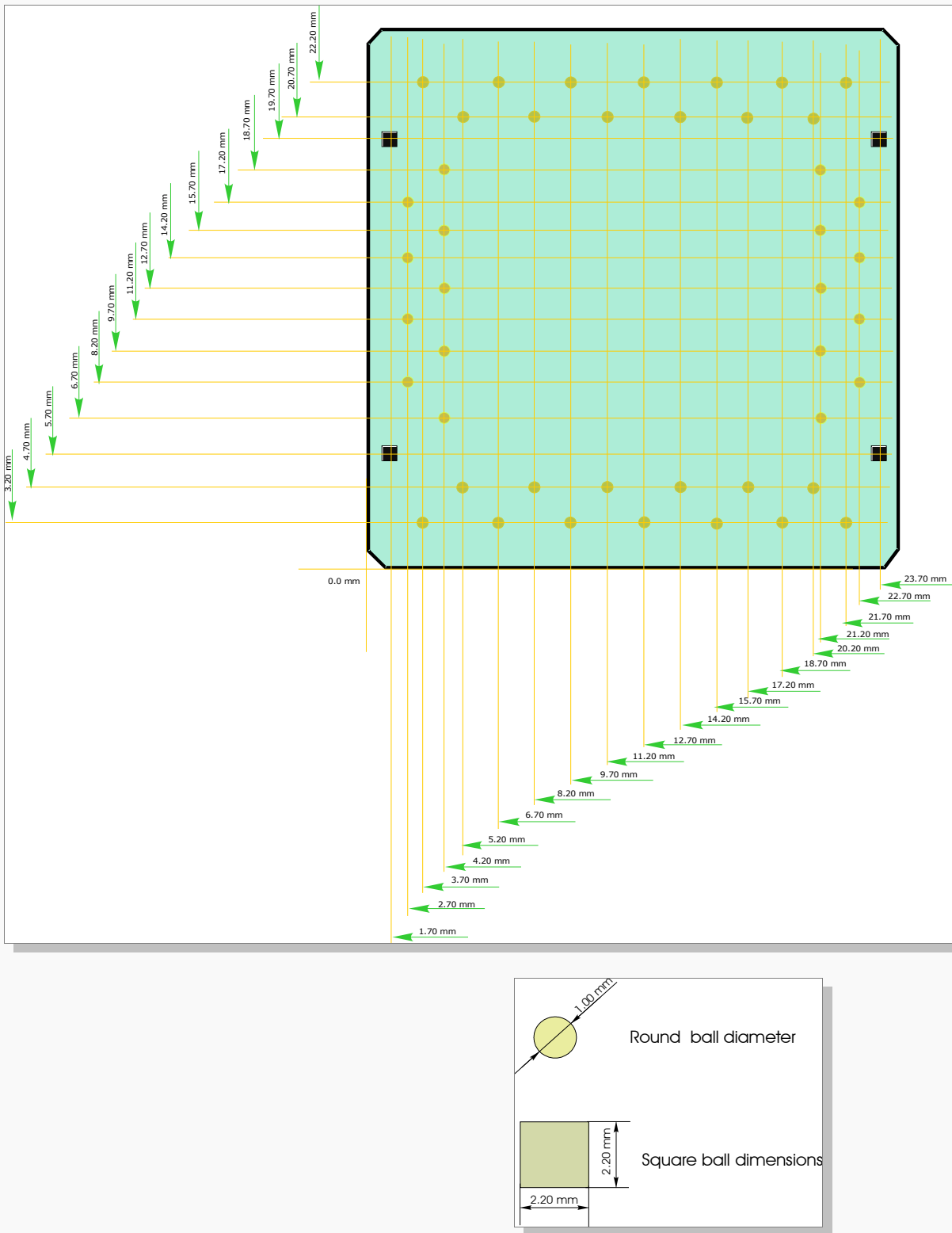
Figure 12: The mechanical draw of the JP13-B-LP receiver
