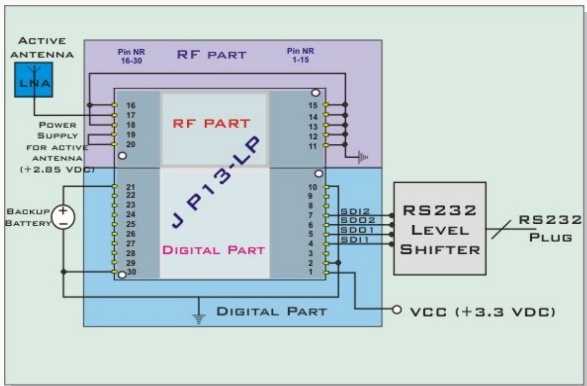
Figure 18: The minimum hardware interface of JP13-LP (with edge contacts) to get started.
