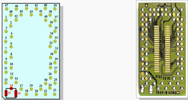
Figure 9: JP13-S-LP ball assignment.
