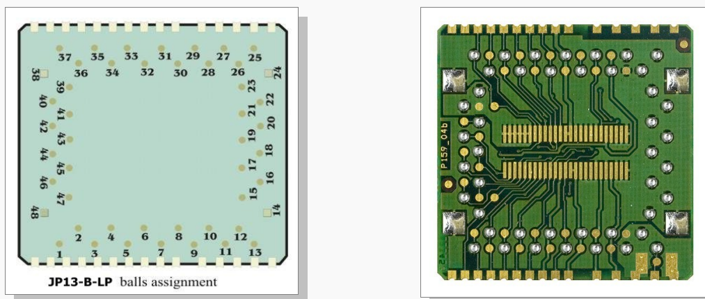
Figure 8: JP13-B-LP ball assignment.
