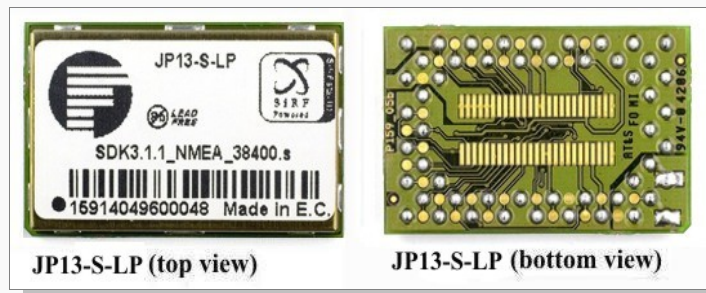
Figure 2: The FALCOM JP13-S-LP version 5b PCB (top and bottom view)
