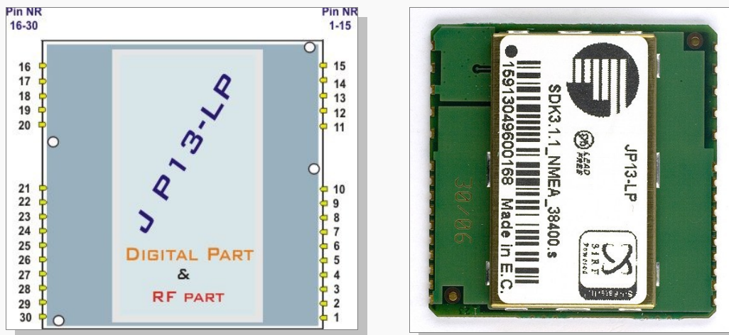
Figure 7: JP13-LP pin out.
