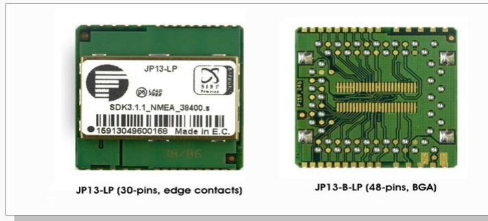
Figure 1: The FALCOM JP13-LP (left) and JP13-B-LP (right) GPS receivers (top and bottom views)
