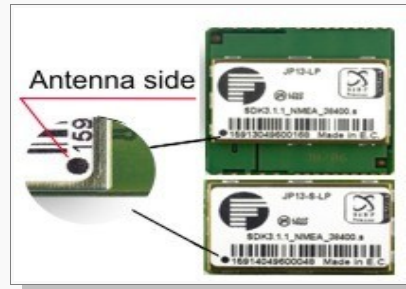
Figure 6: JP13-LP & JP13-S-LP orientation point for antenna site.
