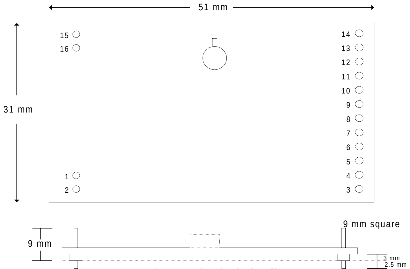
Fig 1 Mechanical detail
